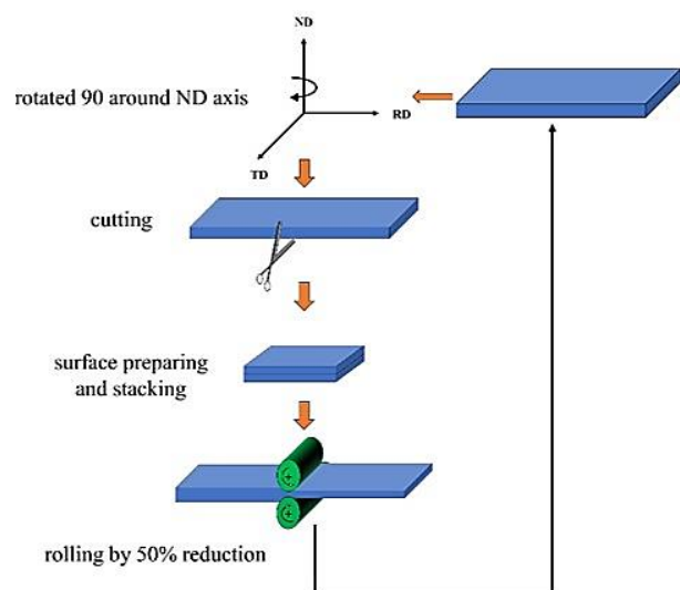
Fig. 2 Schematic illustration of CARB process
